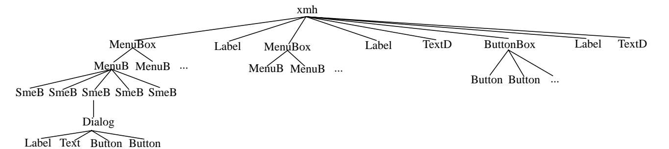
Figure 2b: Corresponding XMH Auditory Interface Component Hierarchy
